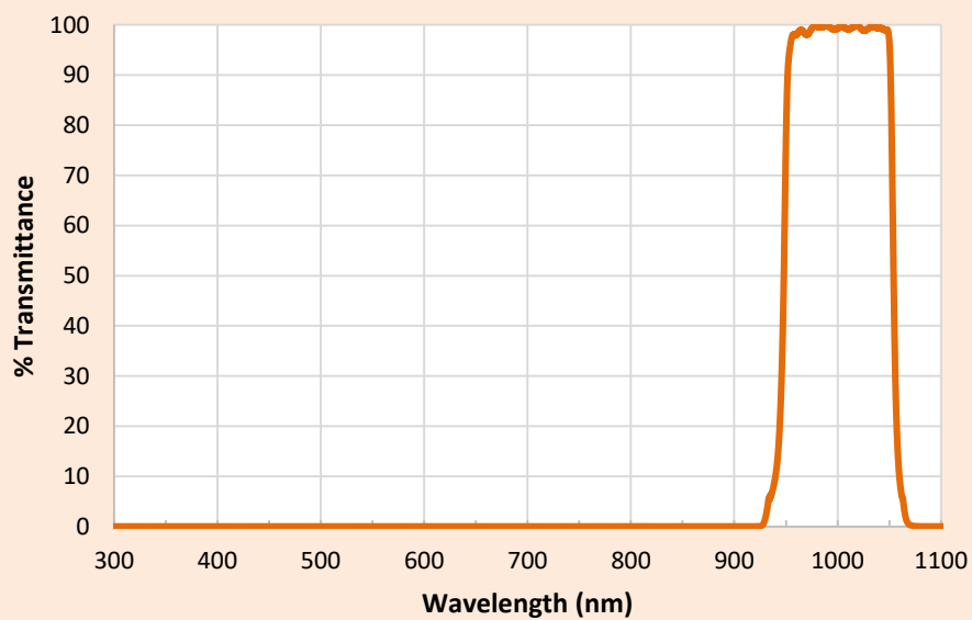
Astrodon Y Photometric Gen 2 Sloan Filter
