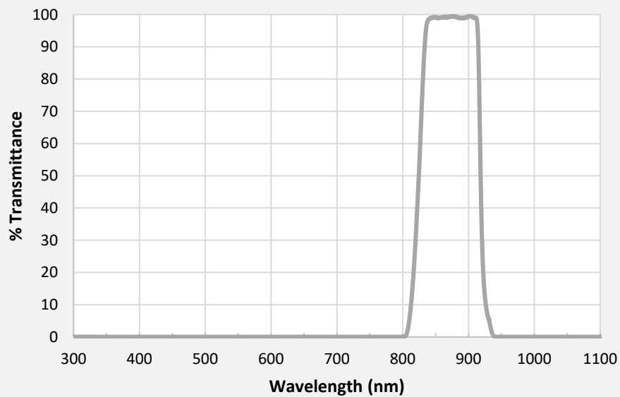
Astrodon z_s Photometric Gen 2 Sloan Filter
