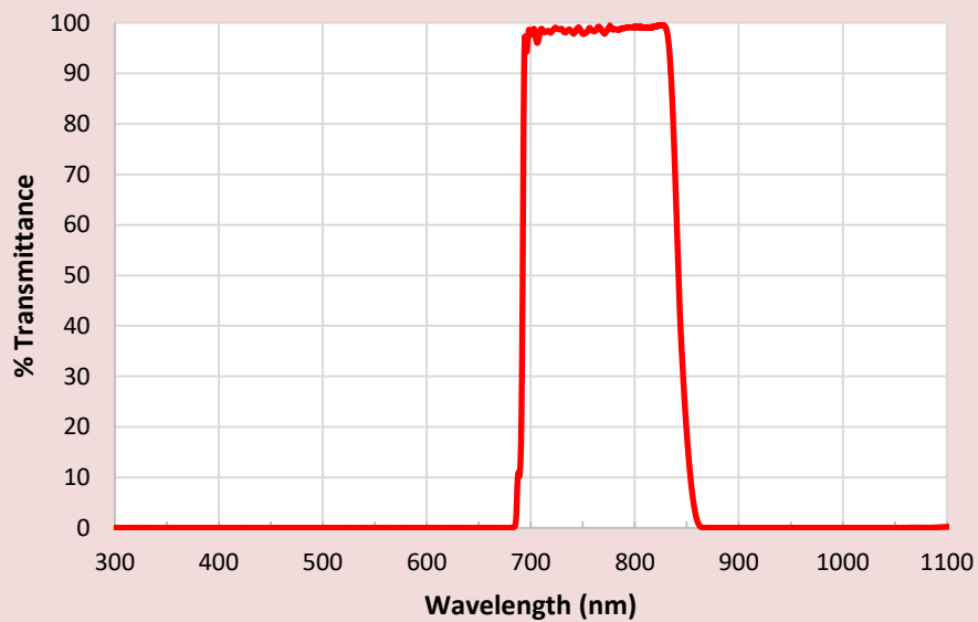
Astrodon i' Photometric Gen 2 Sloan Filter
