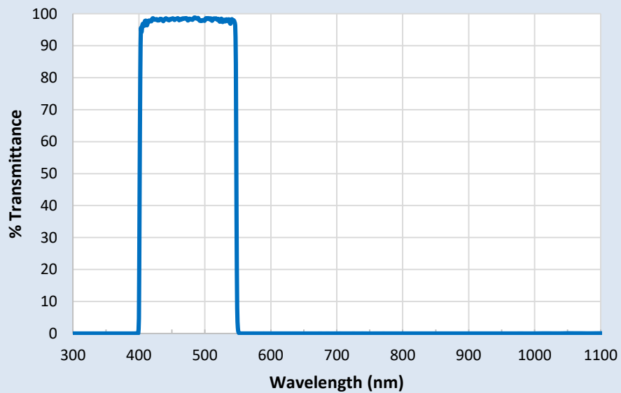
Astrodon g' Photometric Gen 2 Sloan Filter
