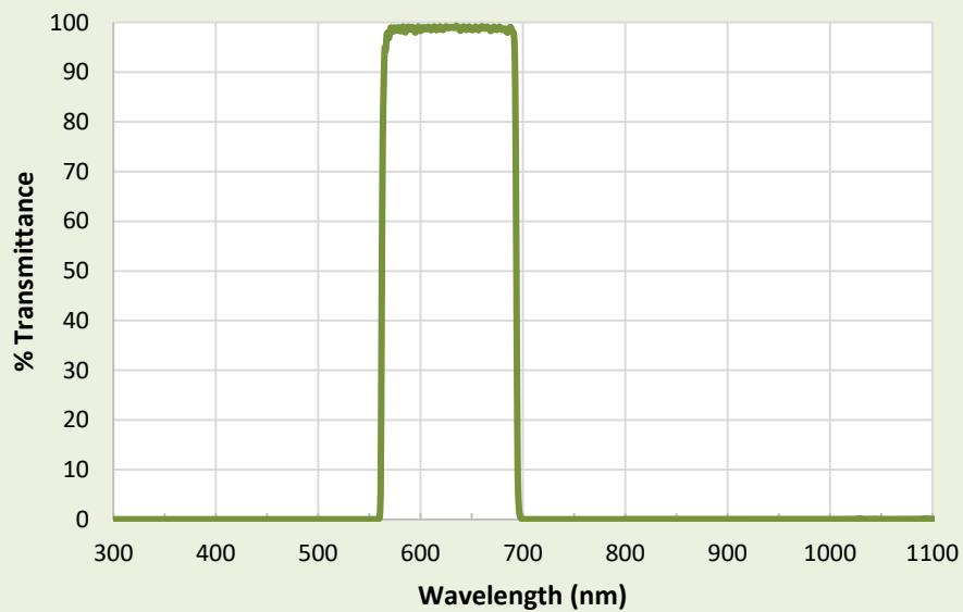
Astrodon r' Photometric Gen 2 Sloan Filter
