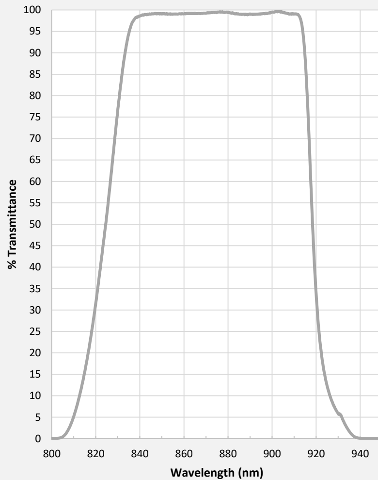
Astrodon z_s Photometric Gen 2 Sloan Filter
