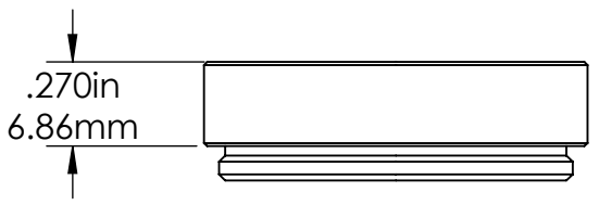
New Astrodon Filter Cell (Production Since Sept 2019)
