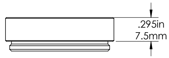
Old Astrodon Filter Cell (Production Prior to 2019)
